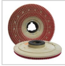
Tufted Stiff Poly Bristle Pad Driver 3/4" long bristles, 3/4" riser #A0047M - 9"
