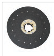
Diamond Pad Driver #A0017DPD - 13" #A0034 - 15" #A0010DPD - 17" #A0011DPD - 20"
