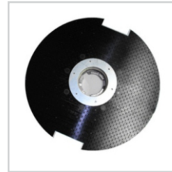
Weighted Diamond Pad Driver Steel Block & Clutch Plate #A0017WTDPD - 12" (25#) #A0010WTDPD - 17" (46#) #A0011WTDPD - 20" (64#)
